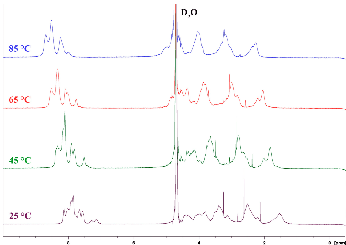
Figure 6. Variable temperature (VT) NMR experiments with [\text{Lu}(\text{C3octapa})]^- ( \text{D}_2\text{O} , 400 MHz), showing broad signals at 25 ^\circ\text{C} most likely arising from fluxional isomers and/or aqua ligand exchange at 25 ^\circ\text{C} , with further broadening and coalescing being observed as the temperature was increased to 85 ^\circ\text{C} in 20 ^\circ\text{C} increments, suggesting fluxional isomerization between multiple isomers was increased elevated temperatures.
