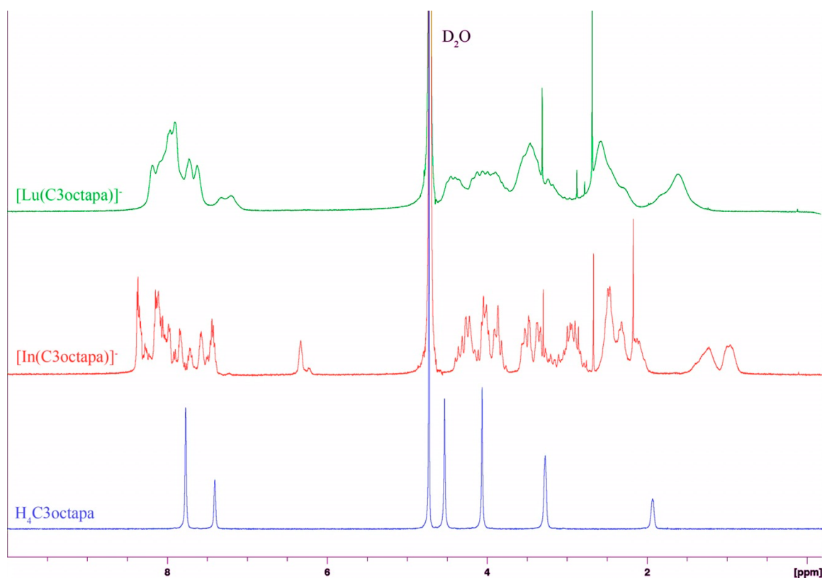
Figure 1. Stacked NMR spectra of H_4C_3octapa ( D_2O , 25 °C, 600 MHz), metal complex [In(C_3octapa)]^- ( D_2O , 25 °C, 400 MHz) showing complicated but sharp signals suggesting multiple static isomers, and [Lu(C_3octapa)]^- ( D_2O , 25 °C, 300 MHz) showing complicated and broad signals suggesting fluxional isomerization.
