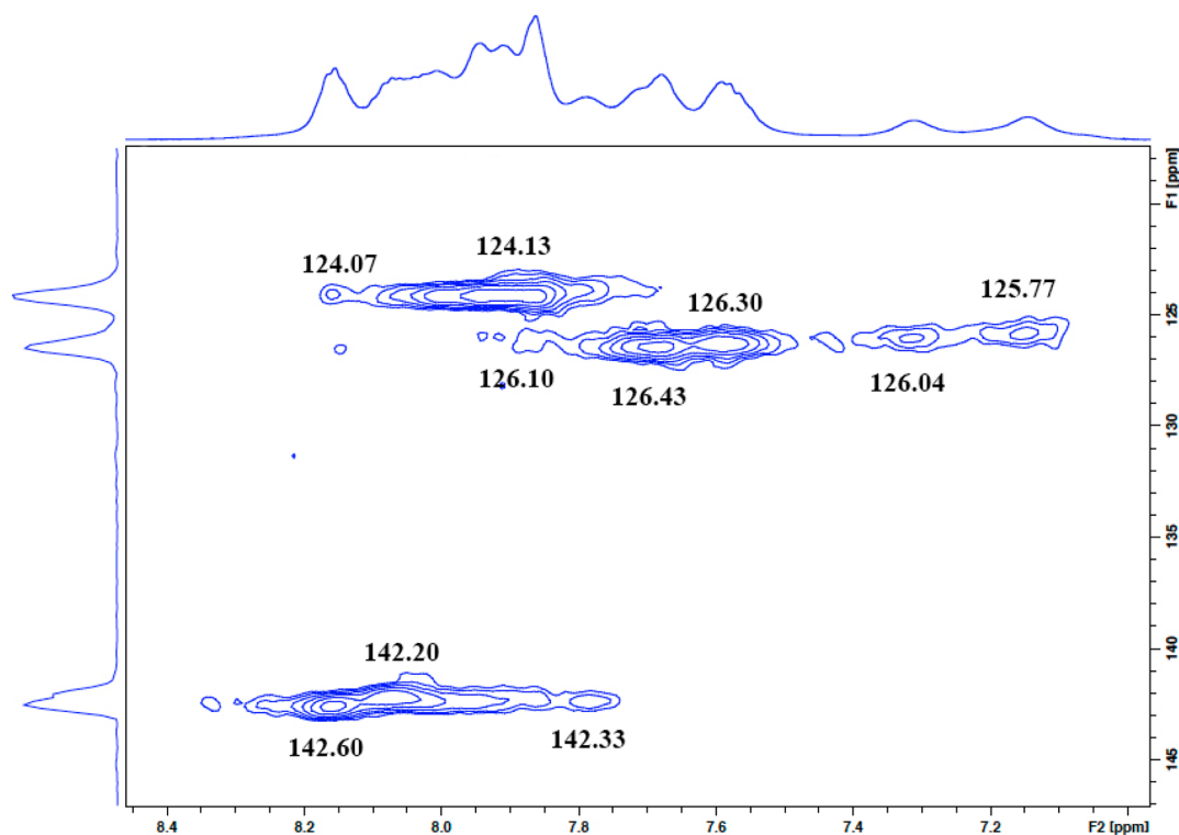
Figure 5. ^1\text{H} - ^{13}\text{C} HSQC NMR (600/150 MHz, \text{D}_2\text{O} , 25 ^\circ\text{C} ) expansion of aromatic signals in spectrum of [\text{Lu}(\text{C3octapa})]^- , showing correlations to 10 unique ^{13}\text{C} signals, with spectral resolution being worse than that of [\text{In}(\text{C3octapa})]^- in Figure 4 due to the broad signals from fluxional isomerization ( ^{13}\text{C} NMR spectra externally referenced to MeOH in \text{D}_2\text{O} ) (for full HSQC spectrum and expansions, see Figures S19 and S20).
